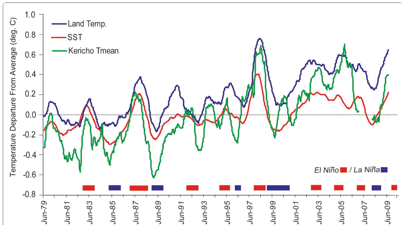
Figure 4 Time series of monthly departures from 1980-2009 mean values (deg. C) with an 11-month moving average applied for Kericho Tmean (green line), global tropical SST (25S-25N) (red line) and tropical land area mean temperature (blue line). Color bars at the bottom of the figure show the occurrence of El Niño and La Niña events (based on the definition in use at the US Climate Prediction Center). See Table 2 for temporal correlations between these variables.
