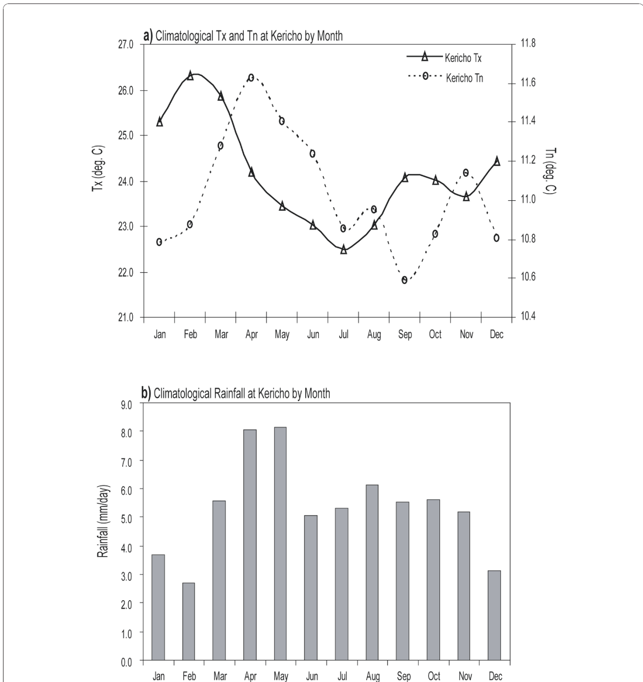
Figure 1 Average monthly climate conditions at Kericho for the period 1980-2009 a) lines indicate monthly average temperature (deg. C) Tx (left axis) and Tn (right axis) b) bars indicate average monthly rainfall (mm/day, left axis).
