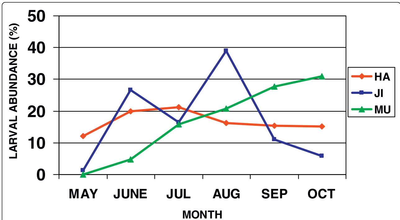
Figure 7 Relative monthly abundance of Anopheles sinensis larvae from rice paddies and irrigation ditches in Munsan (MU), Jinbo (JI) and Hayang (HA), Republic of Korea (May-October 2007).
