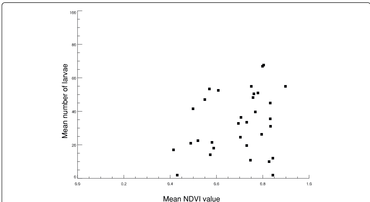
Figure 8 Summary of the relationship between mean NDVI values and mean number of Anopheles larvae collected from various locations in the Republic of Korea. Each point (solid square, n = 33 points) represents the average NDVI value for all collection locations within those sites for a single month (x-axis). This is plotted against the mean number of larvae for all collection locations within the site for that same month (y-axis).
